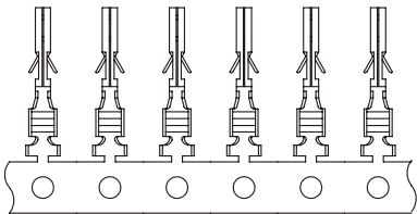
TERNIMAL / female MF300TF - X - XX
