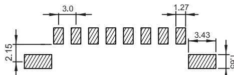
Recommended P.C. Board SMD Layout
