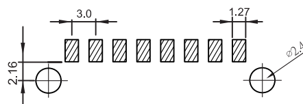
Recommended P.C. Board SMD Layout
