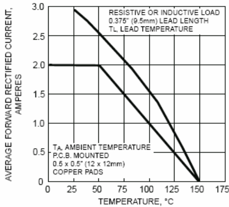
FIG. 1 - MAXIMUM FORWARD CURRENT DERATING CURVES
