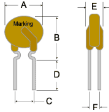
Figure 2 Lead Size : 24AWG, Ø 0.51 mm Diameter
