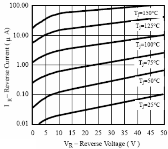
Figure 1. Reverse Current vs. Reverse Voltage
