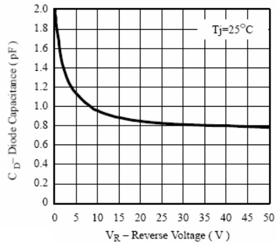
Figure 2. Diode Capacitance vs. Reverse Voltage
