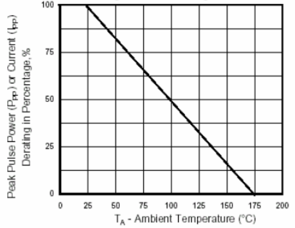
Fig.2-Power Derating Curve
